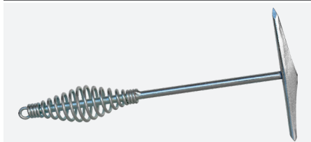
Metal chipping hammer with spring handle
